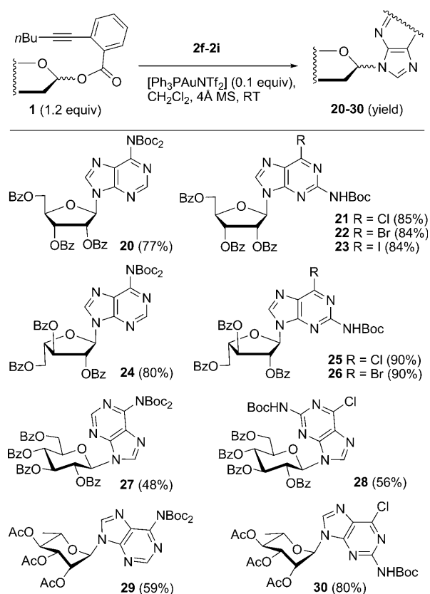
Scheme 3. N-glycosylation of Boc-protected purines 2 f–i with glycosyl ortho -hexynylbenzoates. MS = molecular sieves.
